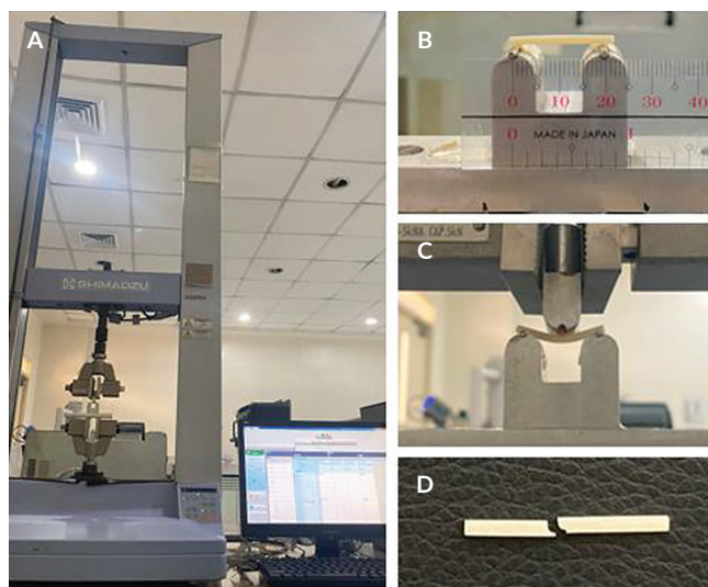
Figure 2. (A) Universal Testing Machine used (AGS-X, Shimadzu, Japan), (B) Support beams 20 mm apart, (C) Three-point bend test; (D) A fractured specimen.
