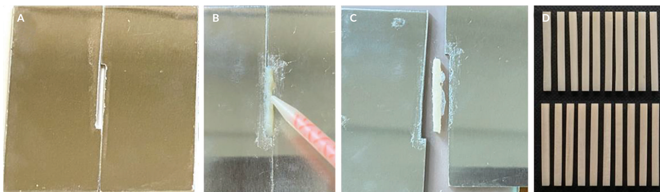
Figure 1. (A) The custom metal mold for specimen fabrication, (B) Dispensing the bis-acryl resin material, (C) A freshly prepared specimen, (D) Actual specimens tested in the study.
