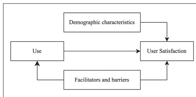
Figure 2. Conceptual framework.
