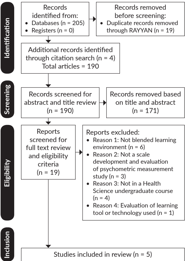
Figure 2. PRISMA Flowchart.
